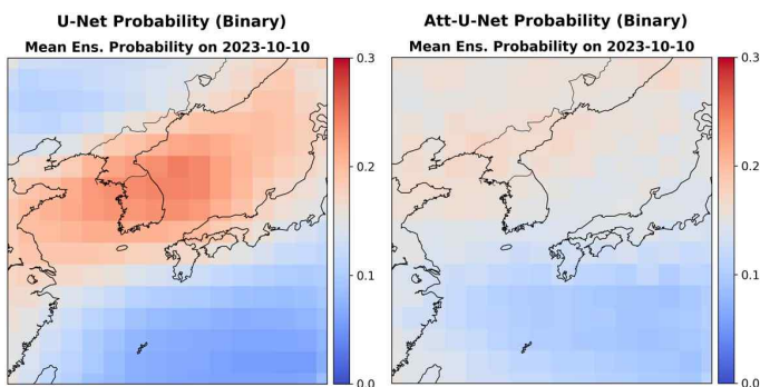
Figure 3.18 This figure shows the averaged probabilities from 11 ensemble predictions produced by deep learning models trained on binary labels of 3-week mean maximum temperature. The left panel displays results from the U-Net model, while the right panel shows corresponding outputs from the Attention U-Net model for 10 October 2023.
