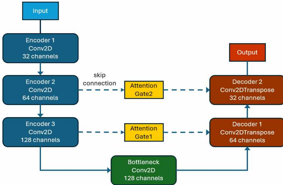
Figure 2.6 Attention-Enhanced U-Net Architecture Overview. The diagram illustrates an encoder-decoder U-Net architecture augmented with attention gates that refine skip-connection features. It shows how multi-scale encoded features pass through attention modules before being merged with decoder layers to produce the final output.
