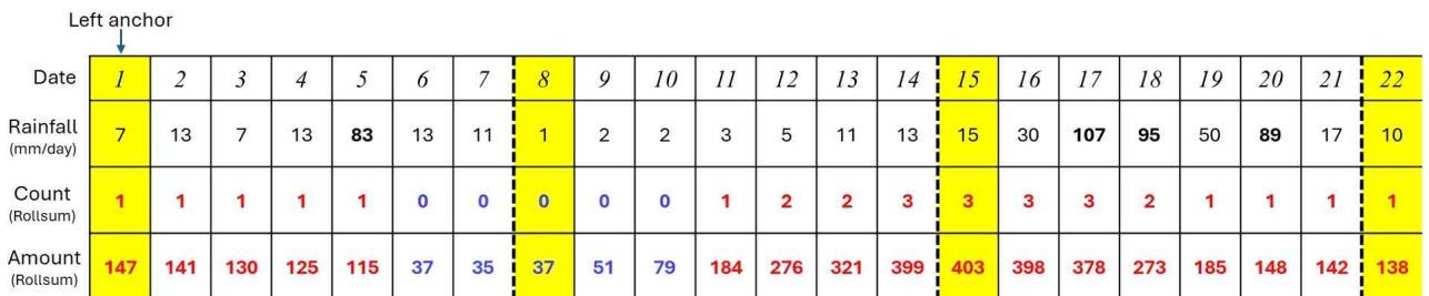
Figure 2.4. Example of how weekly rolling sum on daily rainfall works. Rainfall amount (mm/day) shown in bold is the extreme event that exceeds 90th percentile threshold. Figures shown in red are the extreme cases, and those in blue are the non-extreme cases.
