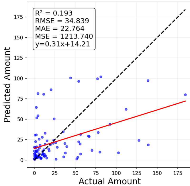
Figure 3.33. Scatter plot of rainfall amount at a 4-week lead predicted by the final model for Seoul grid point compared to actual amount.
