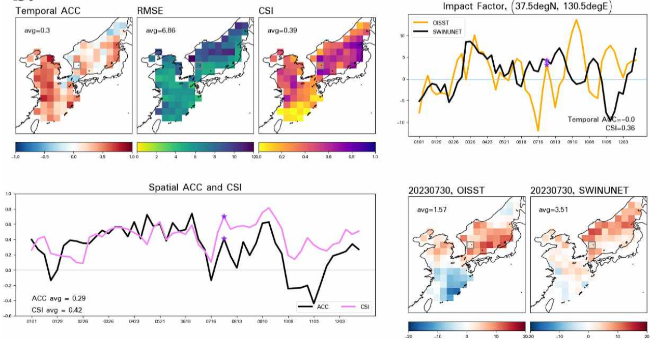
Figure 3.56 Performance of the two best AI models: weekly evaluation of 3-week lead marine heatwave predictions throughout 2023. (a) shows a swinUNet model with the 3Wseq/S2.5/wFOS/RD_added/2:1 train/validation ratio setup, while (b) presents a model with the same configuration but using a 3:1 train/validation ratio. Details are the same as in Figure 3.55.
