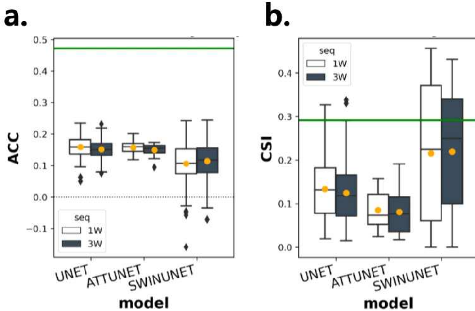
Figure 3.50 Boxplots showing the distribution of (a) ACC and (b) CSI across three models (Base UNet, Attention UNet, and Swin-Transformer UNet) along the x-axis. Colors indicate the temporal sequence of input data (white boxes for one-week inputs and navy boxes for three-week inputs). The green horizontal line represents the ECMWF marine heatwave forecast skill at a 3-week lead time.
