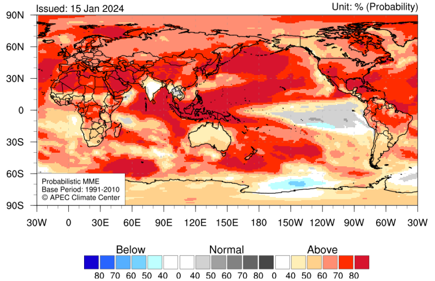
Precipitation for May-July 2025
