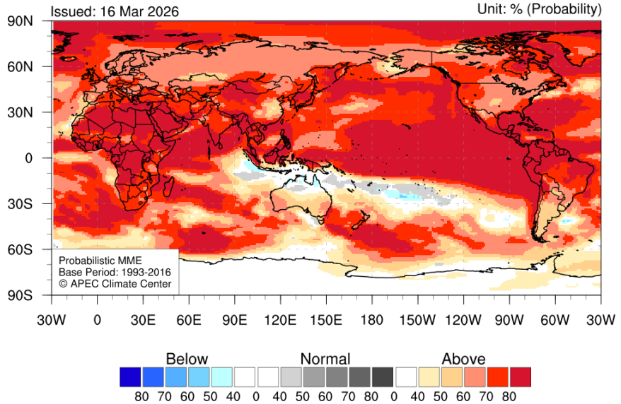
Precipitation for July-September 2026
