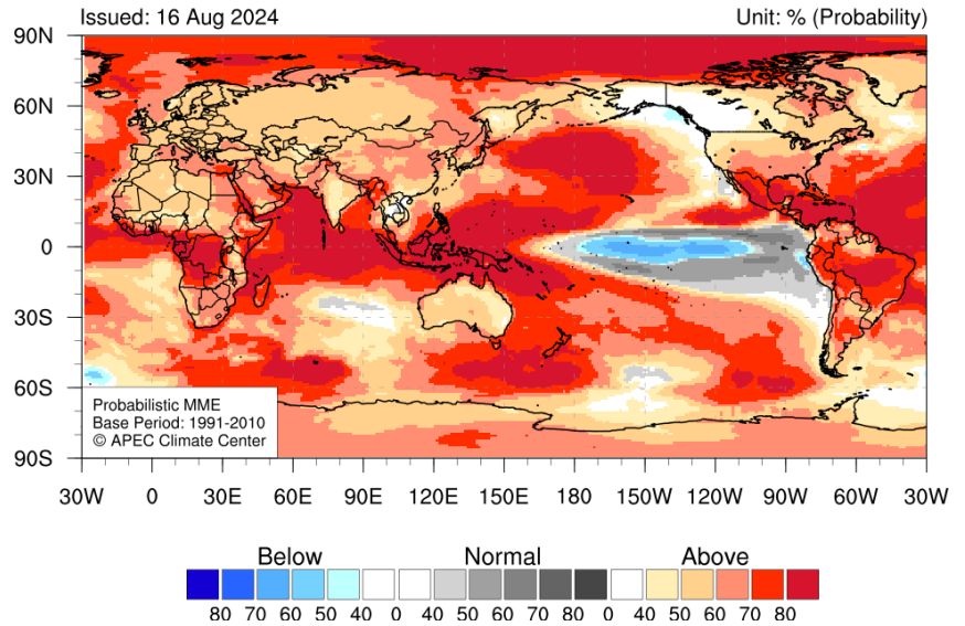
Temperature at 2m for December 2024-February 2025
