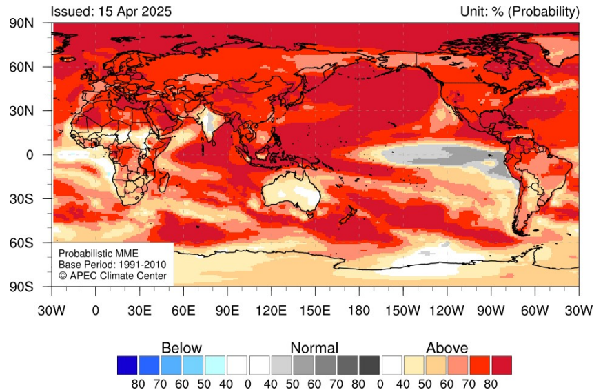
Temperature at 2m for August-October 2025
