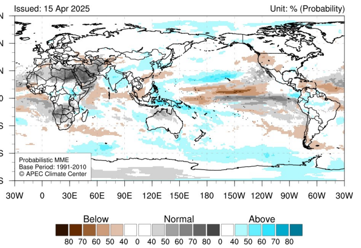
Precipitation for July 2025
